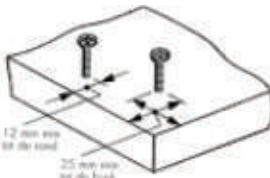
Self Tapping Screw
